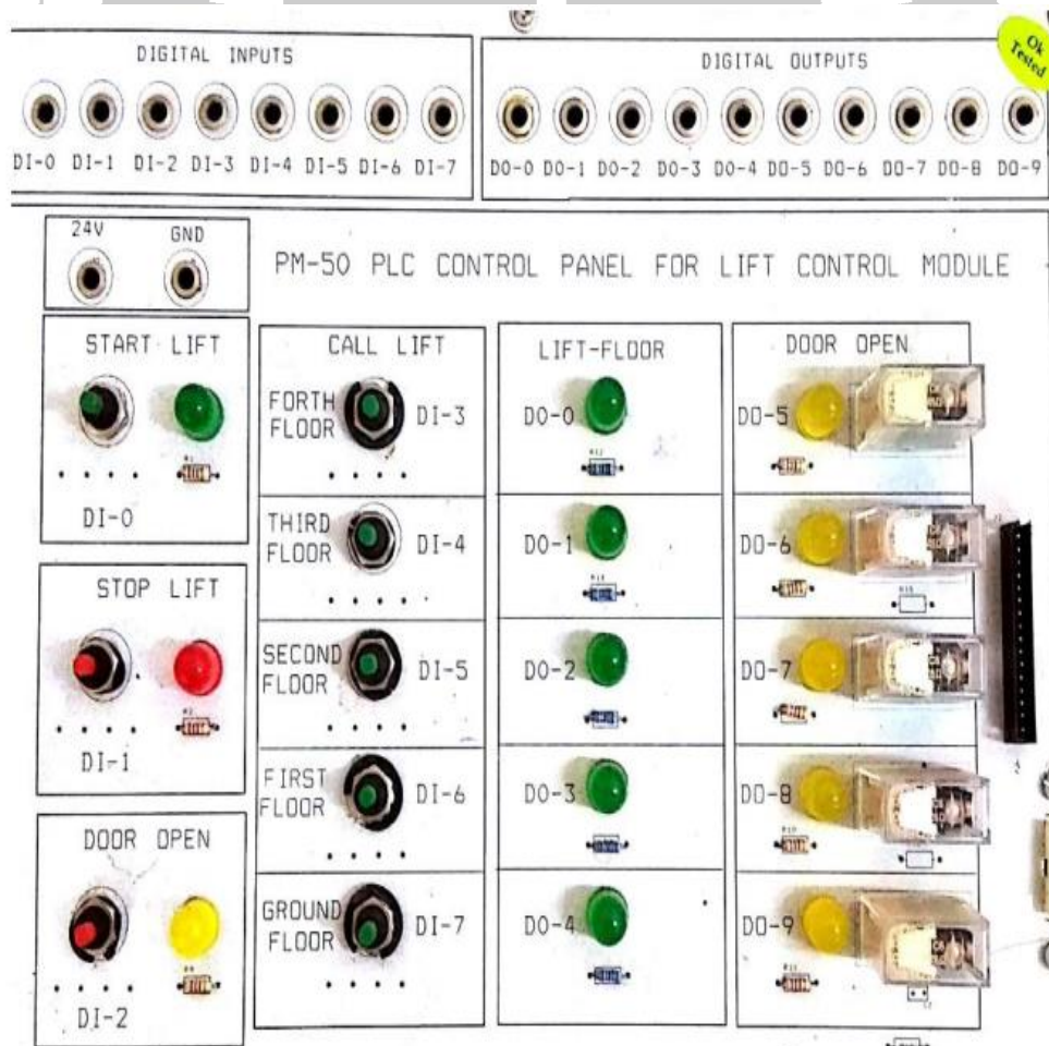
Fig 10.2 Sample Lift / Elevator controller module.
