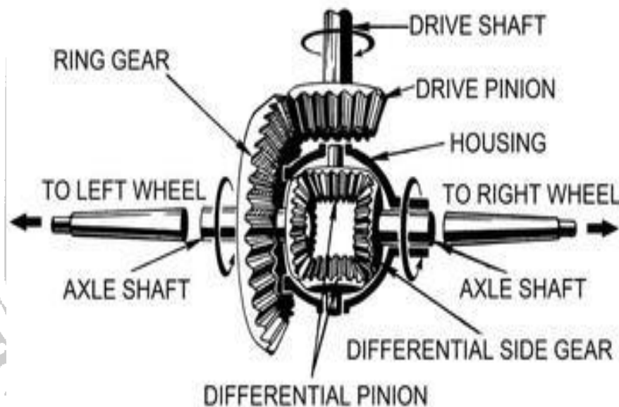
Fig.5.1 Differential Assembly
