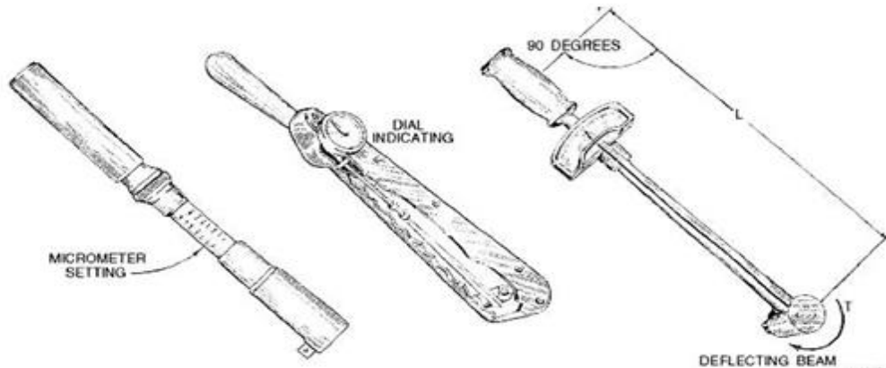
Fig. 2.12 Torque Wrench
