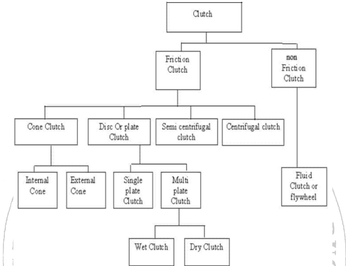
Fig.3.1 Types of Clutch
