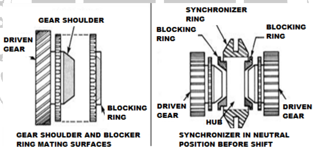
Fig.4.2 Synchronizer Device
